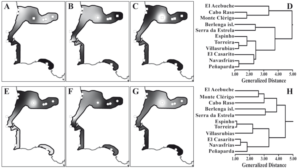
Fig. 3. IDW interpolation maps produced for the first three canonical variates of biometric variation and UPGMA phenograms based on the corresponding generalized distances between populations for male (top) and female (bottom) P. carbonelli . A, E: first canonical variate, B, F: second canonical variate, C, G: third canonical variate. In interpolation maps, lighter colours represent higher values and darker colours, lower values.
