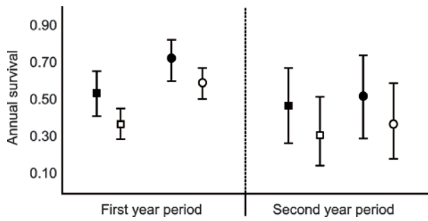
Fig. 1. Average and 95% confidence intervals for survival estimations in sand-dune lizards. Squares: males; circles: females; black: adults; white: juveniles.
