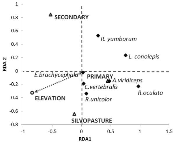
Fig. 2. Redundancy Analysis (RDA) biplot for the 7 species of leaf-litter lizards. RDA 1 and 2 combined account for 94.7% of the variance in the dataset. *one individual only.
