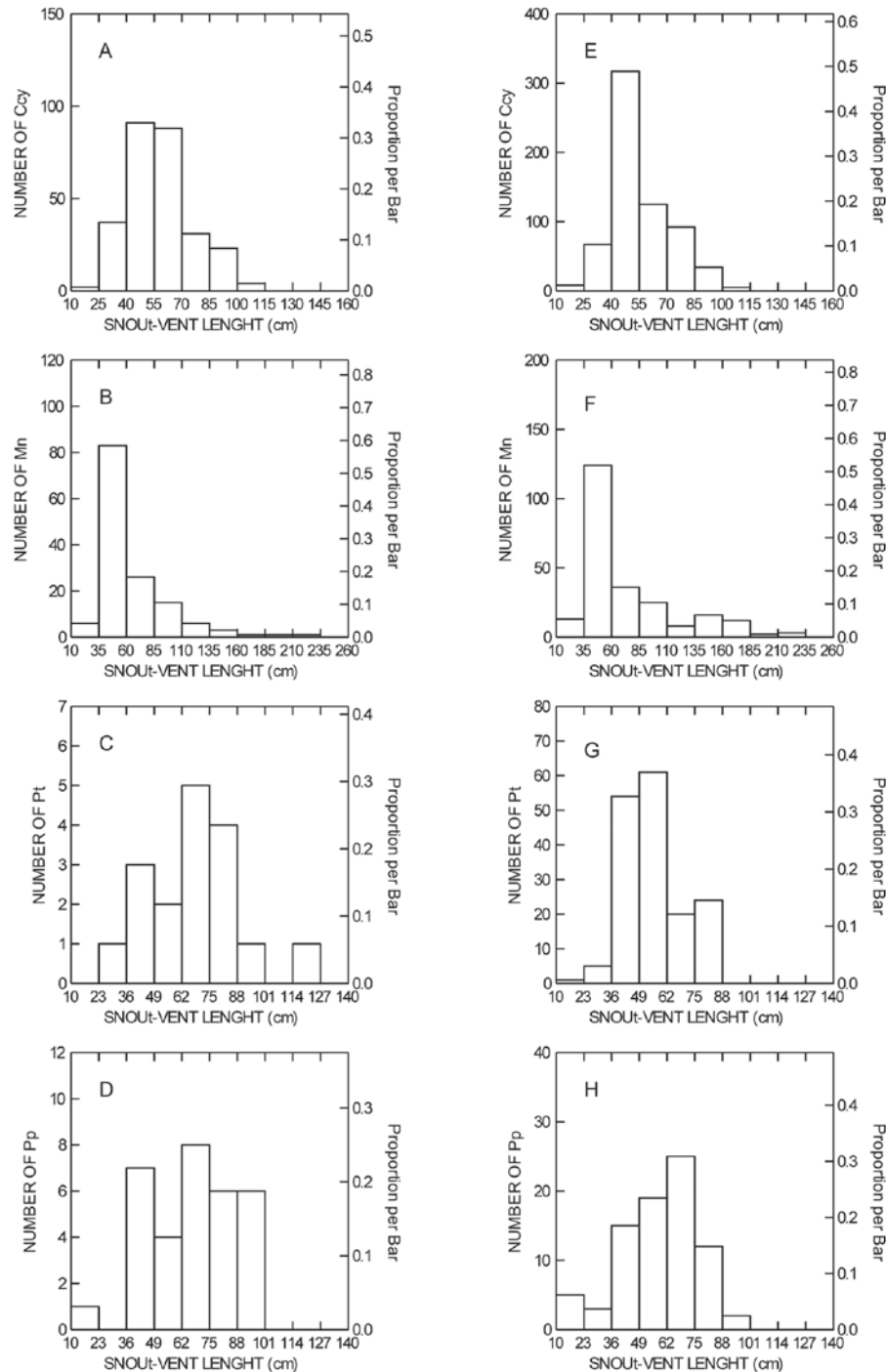
Figure 3. Size structure of caimans before (A, B, C, D) and after filling (E, F, G, H) of the Santo Antônio reservoir. Ccy = C. crocodilus yacare , Mn = M. niger , Pt = P. trigonatus , Pp = P. palpebrosus .
